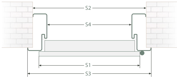
Corner assembly:
